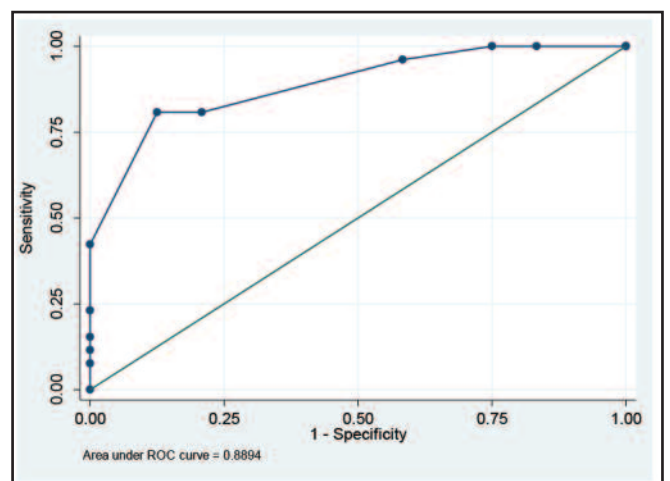
Fig. 2: ROC curve for (SI 2) versus outcome = death
