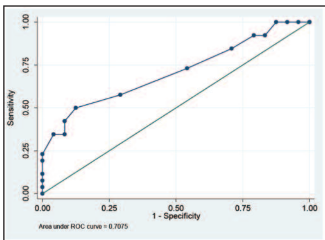
Fig. 1: ROC curve for (SI 1) versus outcome = death
